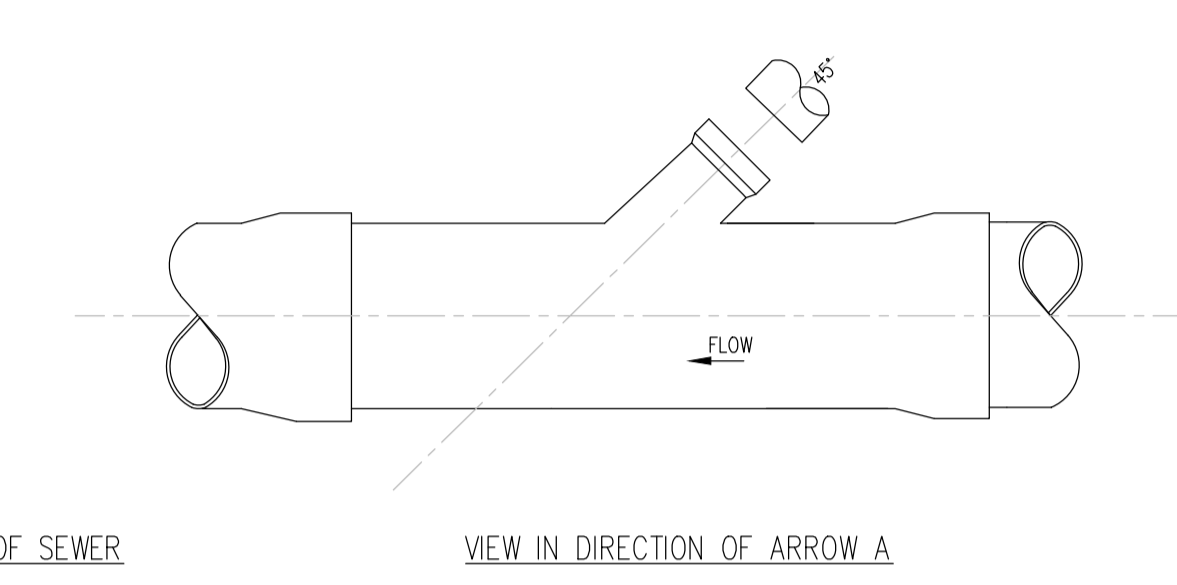
TYPICAL SEWER/SERVICE PIPE (STD-WW-04) SCALE 1:20
